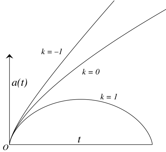
Figure 7: The Robertson-Walker universe with \Lambda = 0 , for k = 1 , k = 0 , and k = -1 .
