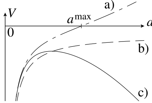
Figure 6: The potential (14.22) for the cases a) k = 0 , \Lambda < 0 , b) k = -1 , \Lambda = 0 and c) k = 0 , \Lambda > 0 . In the case (a), there is a turning point at a = a^{\max} .
