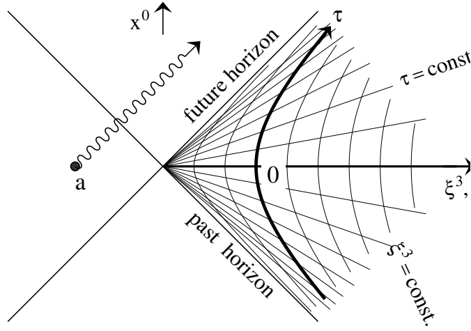
Figure 1: Rindler Space. The curved solid line represents the floor of the elevator, \xi^3 = 0 . A signal emitted from point a can never be received by an inhabitant of Rindler Space, who lives in the quadrant at the right.
